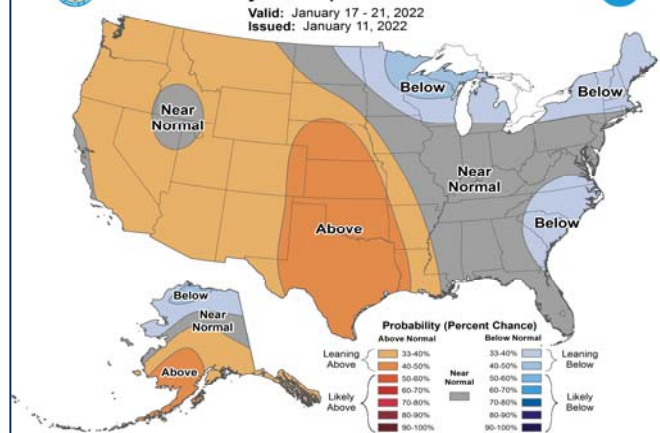
6-10 Day Temperature Outlook
